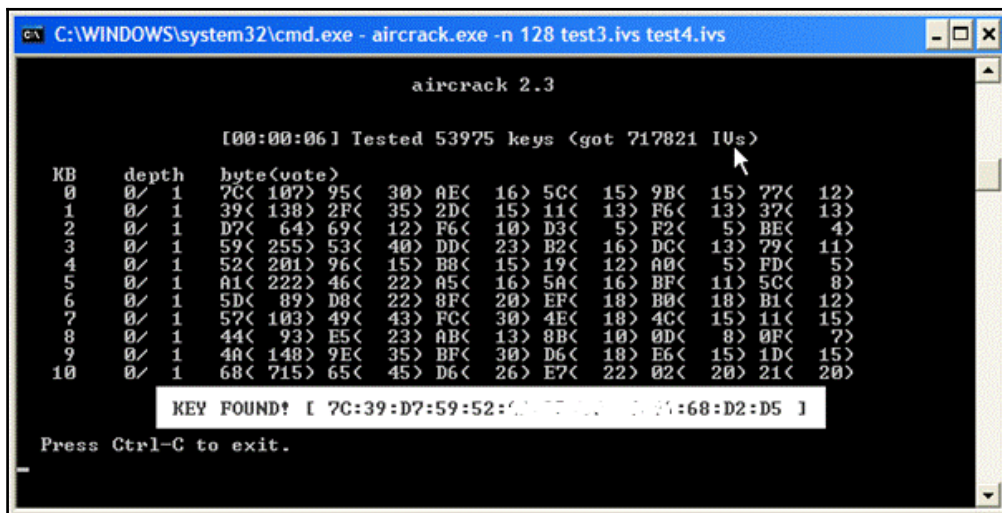
Figure 7: Aircrack-ng interface
