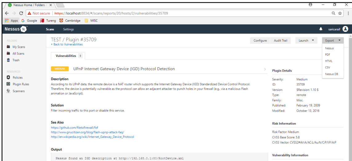
Figure 10 - Exporting results
